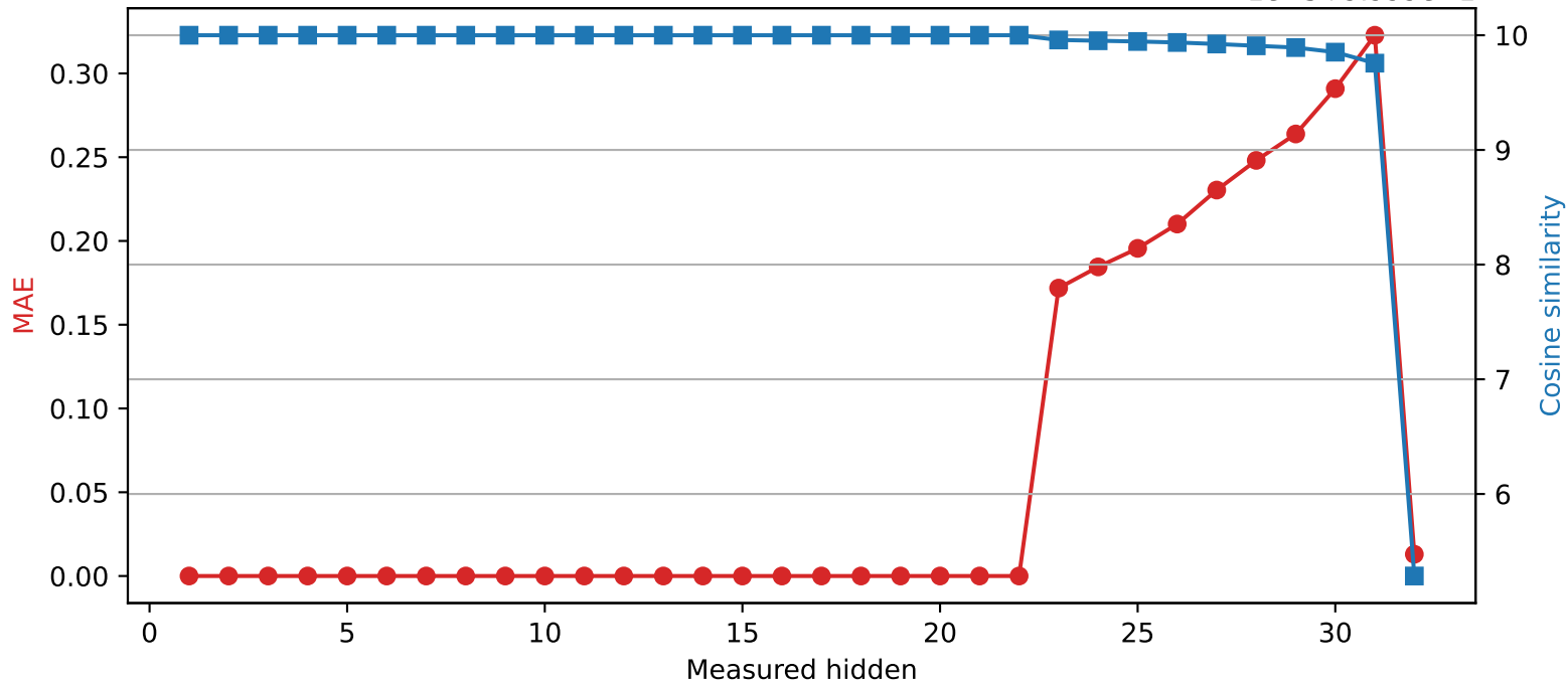
SmolLM2-360M | Quantized layer 22 | float16 \rightarrow int8 1e-5+9.999e-1
