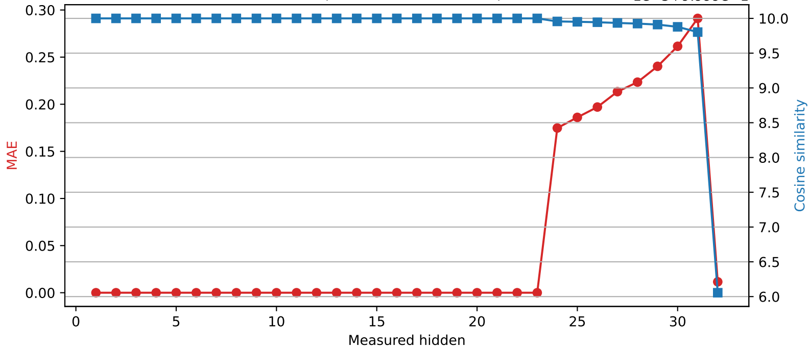
SmolLM2-360M | Quantized layer 23 | float16 \rightarrow int8 1e-5+9.999e-1
