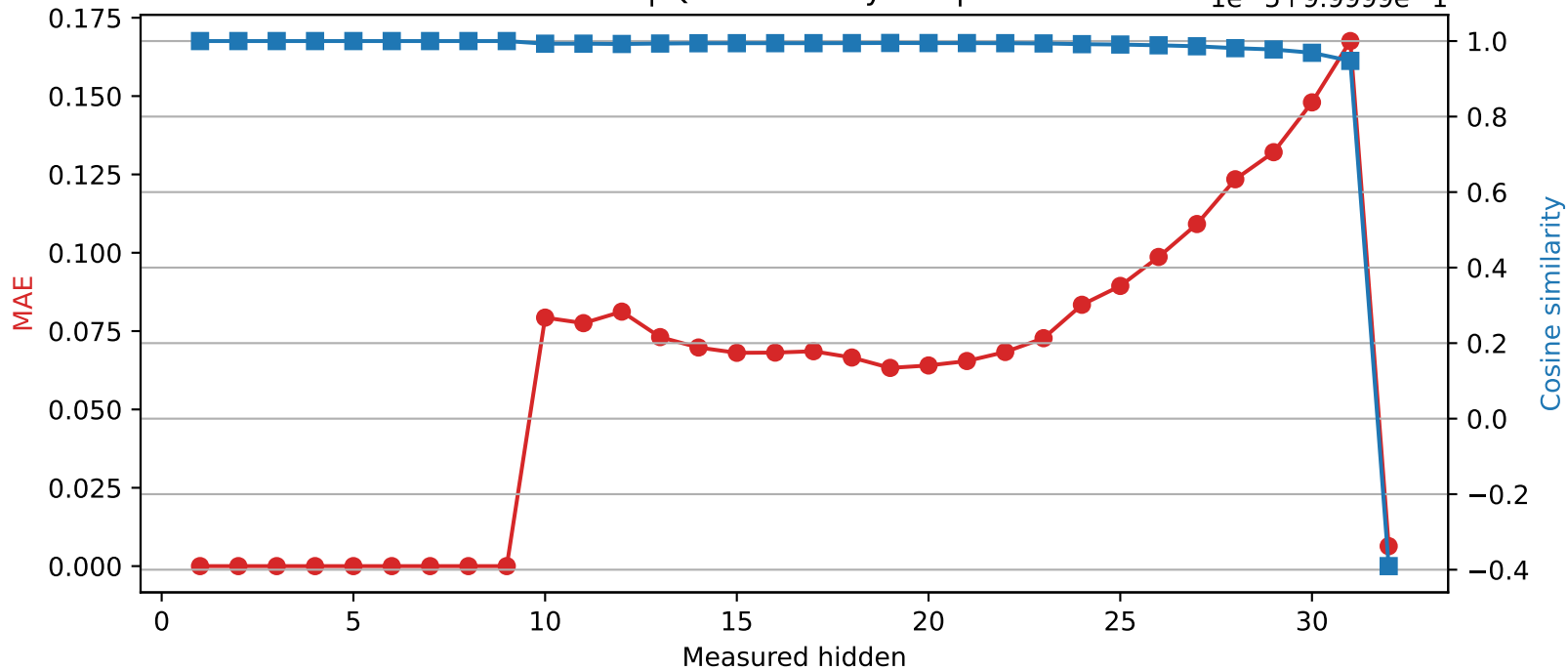
SmolLM2-360M | Quantized layer 9 | float16 \rightarrow int8 1e-5+9.9999e-1
