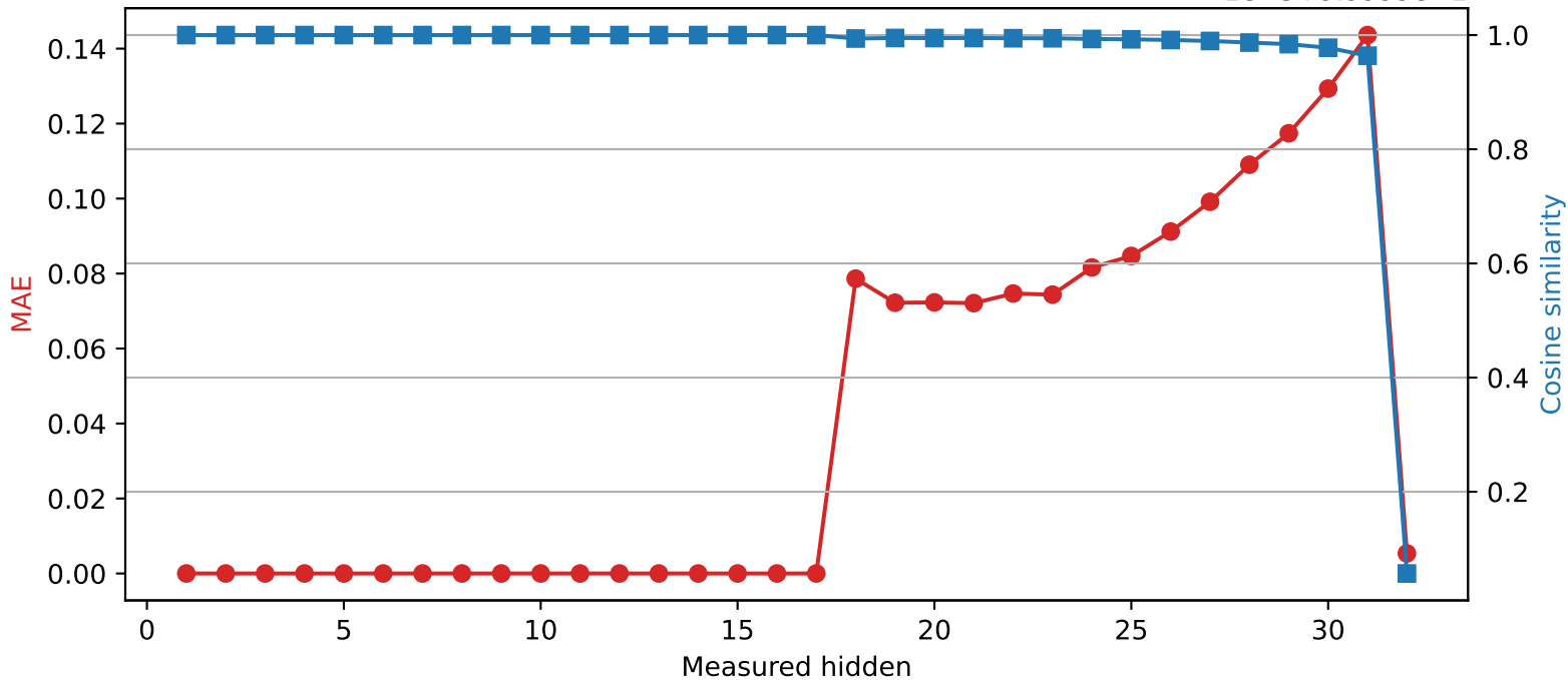
SmolLM2-360M | Quantized layer 17 | float16 \rightarrow int8 1e-5+9.9999e-1
