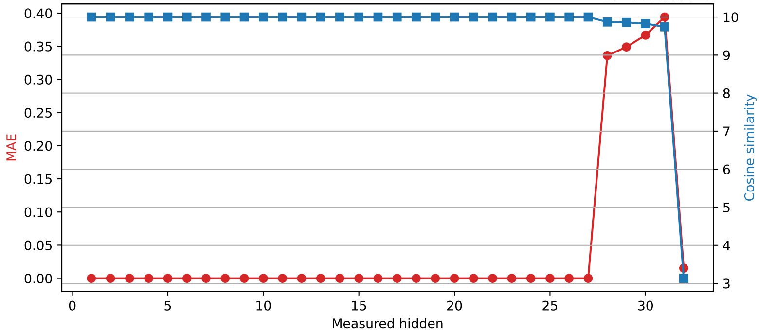
SmolLM2-360M | Quantized layer 27 | float16 \rightarrow int8 1e-5+9.999e-1
