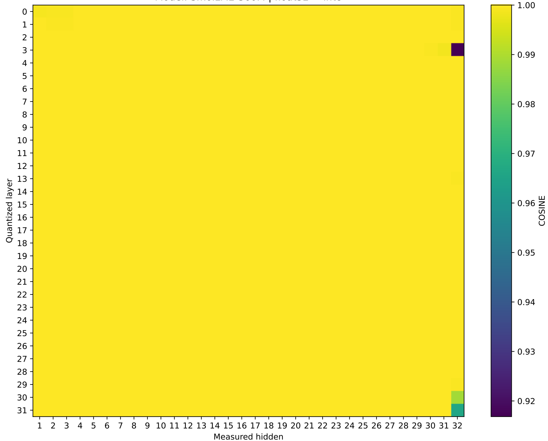
Model: SmolLM2-360M | float32 → int8
