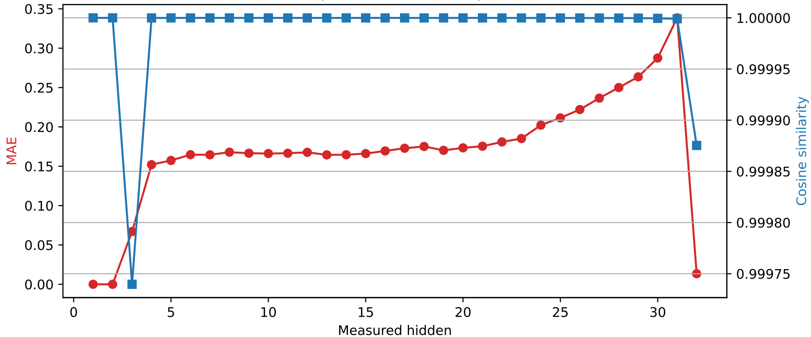
SmolLM2-360M | Quantized layer 2 | float32 → int8
