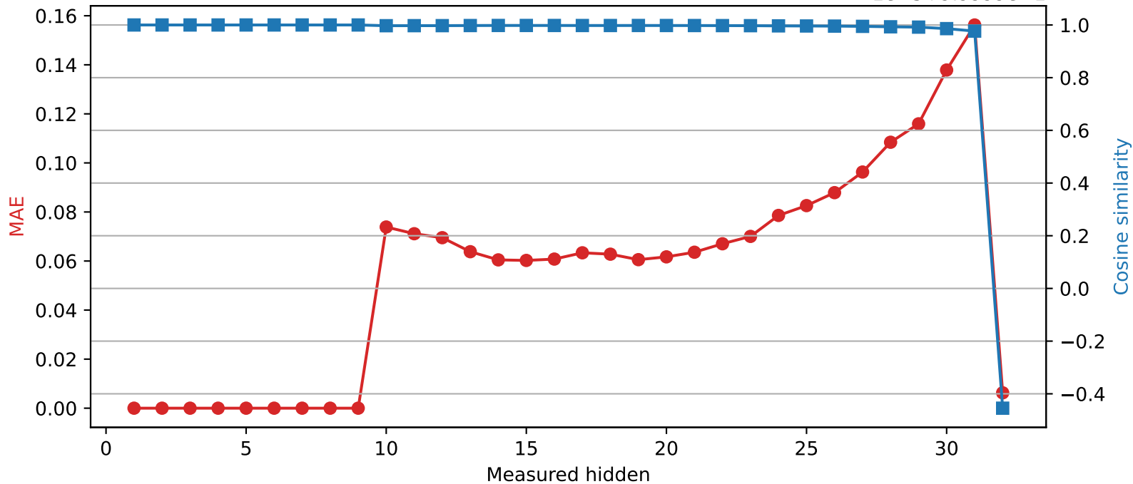
SmolLM2-360M | Quantized layer 9 | float32 \rightarrow int8 1e-5+9.9999e-1
