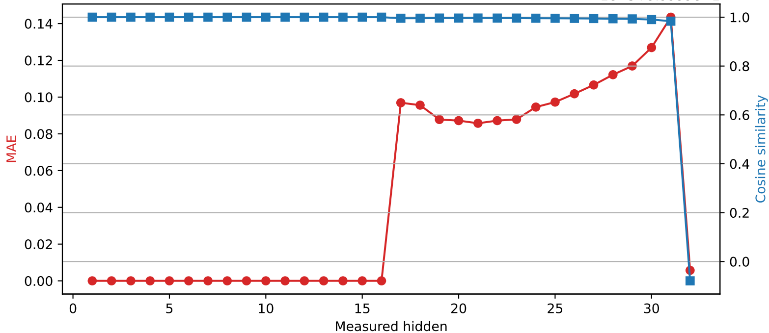
SmolLM2-360M | Quantized layer 16 | float32 \rightarrow int8 1e-5+9.9999e-1
