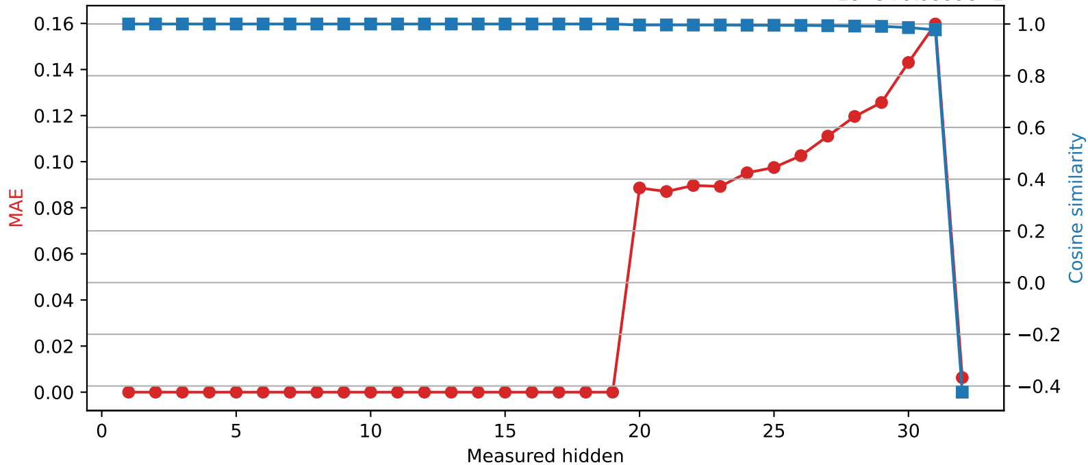
SmolLM2-360M | Quantized layer 19 | float32 \rightarrow int8 1e-5+9.9999e-1
