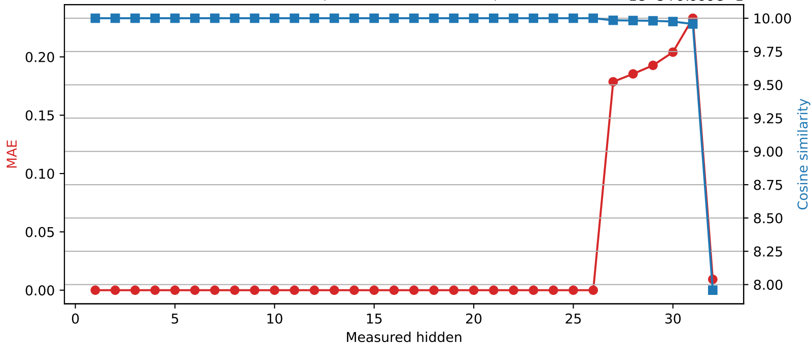
SmolLM2-360M | Quantized layer 26 | float32 → int8 1e-5 + 9.999e-1
