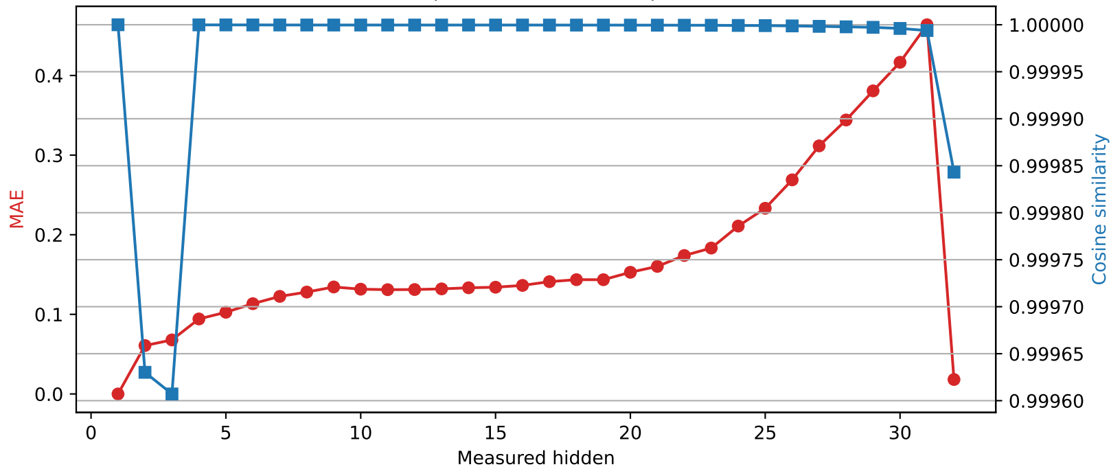
SmolLM2-360M | Quantized layer 1 | float32 → int8
