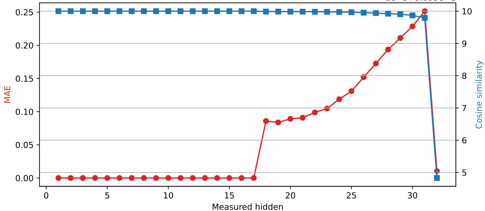
SmolLM2-360M | Quantized layer 17 | float32 → int8 1e-5+9.999e-1
