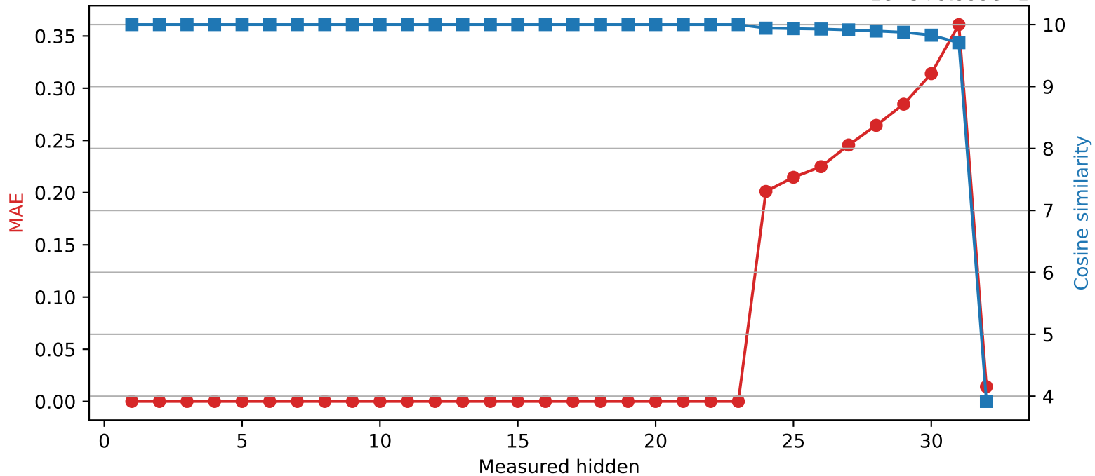
SmolLM2-360M | Quantized layer 23 | float32 → int8 1e-5+9.999e-1
