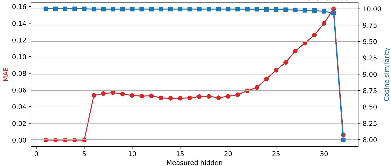
SmolLM2-360M | Quantized layer 5 | float32 → int8
