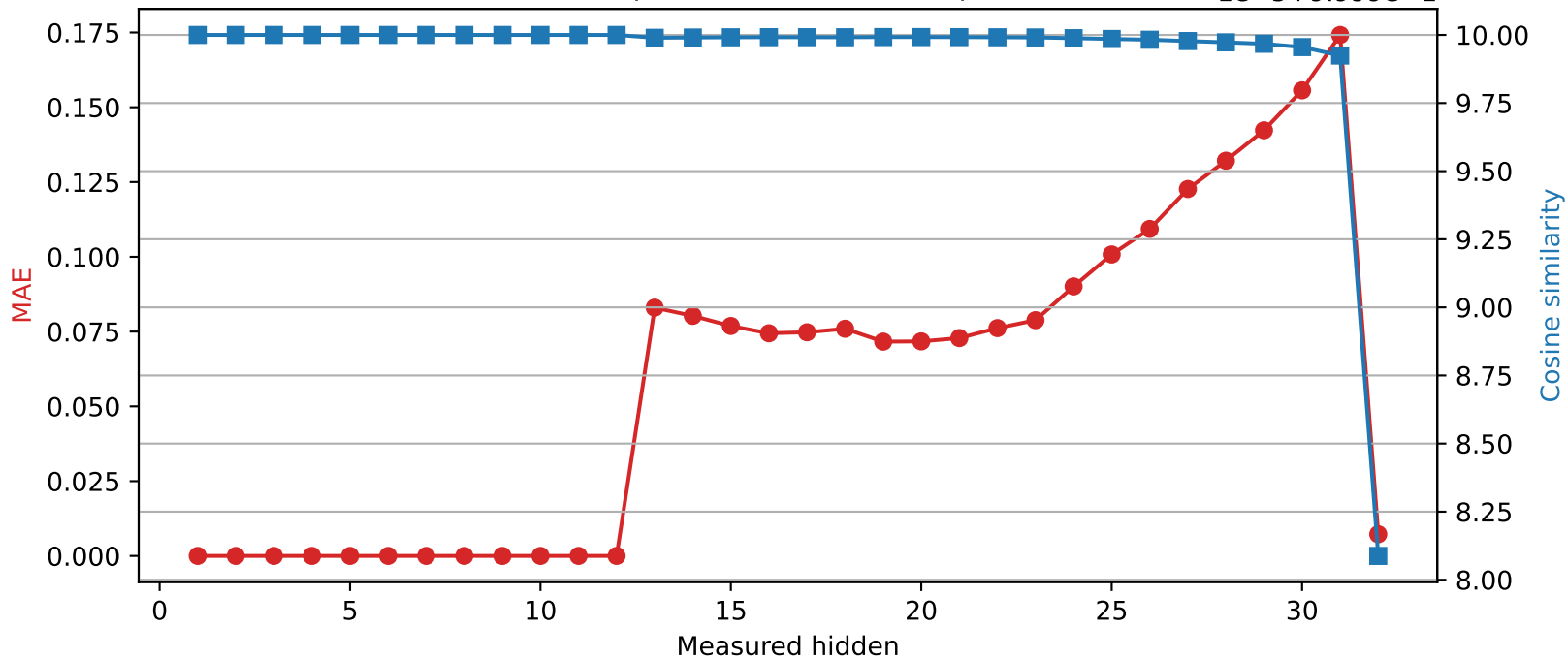
SmolLM2-360M | Quantized layer 12 | float32 → int8 1e-5+9.999e-1
