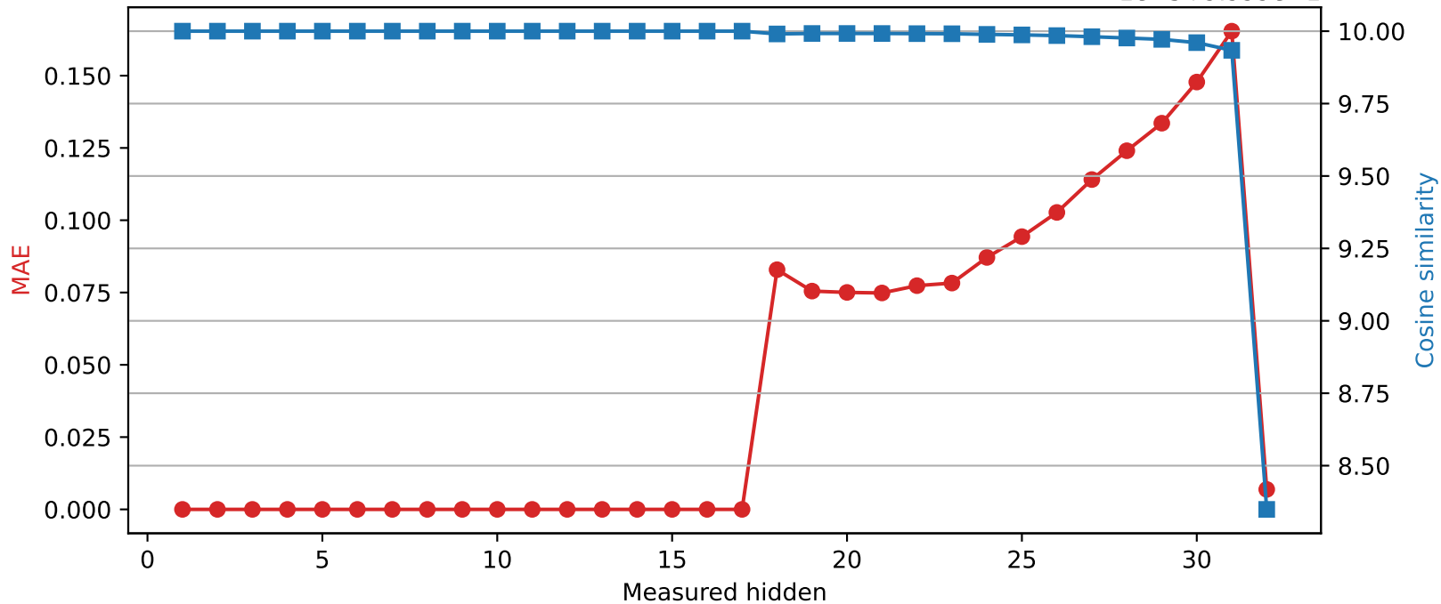
SmolLM2-360M | Quantized layer 17 | float32 → int8 1e-5 + 9.999e-1
