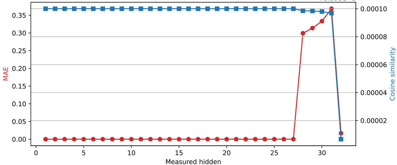
SmolLM2-360M | Quantized layer 27 | float32 \rightarrow int8
