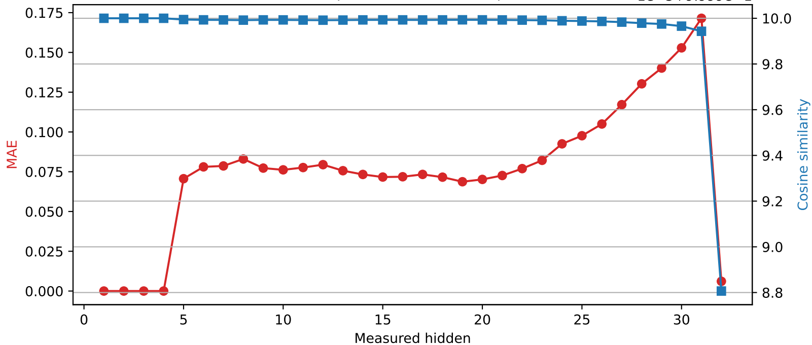
SmolLM2-360M | Quantized layer 4 | float32 → int8
