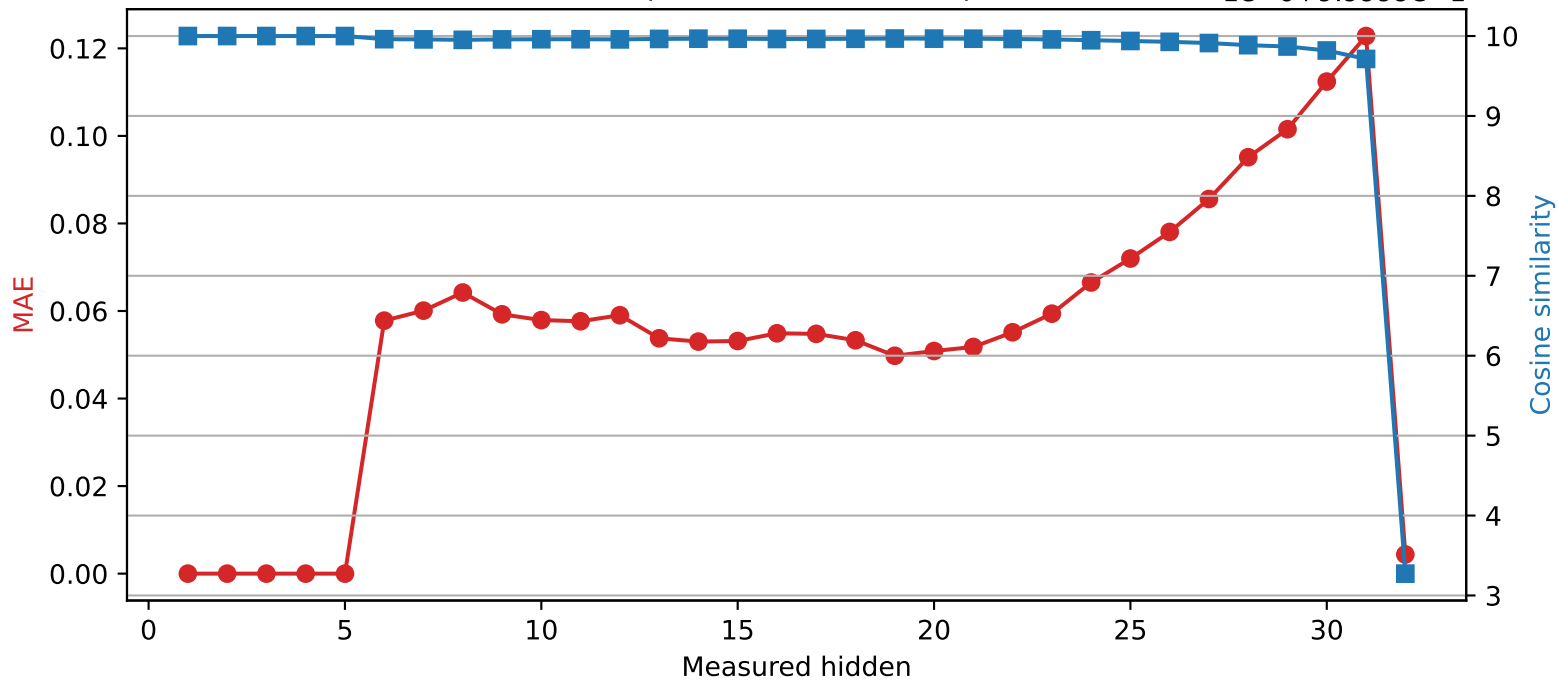
SmolLM2-360M | Quantized layer 5 | float32 \rightarrow int8 1e-6+9.9999e-1
