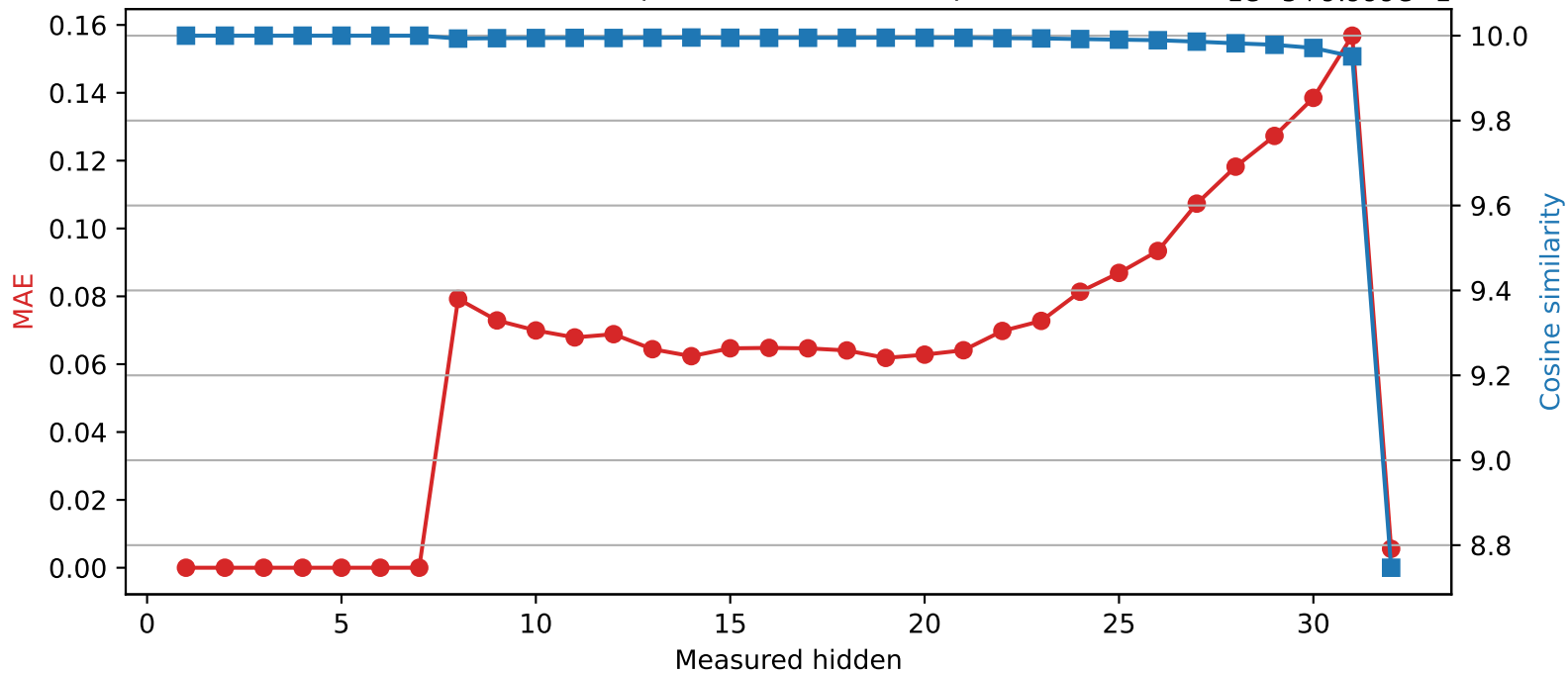
SmolLM2-360M | Quantized layer 7 | float32 → int8
