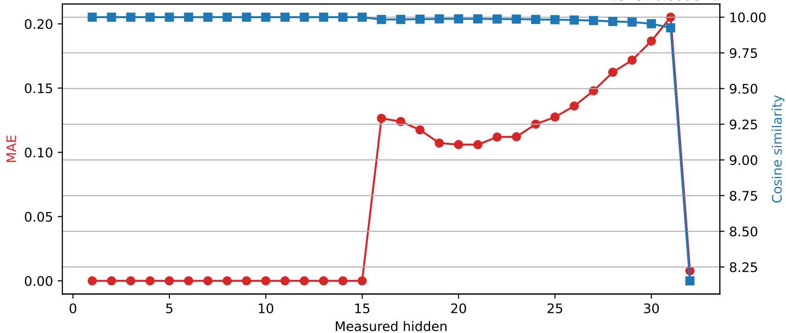
SmolLM2-360M | Quantized layer 15 | float32 \rightarrow int8 1e-5+9.999e-1
