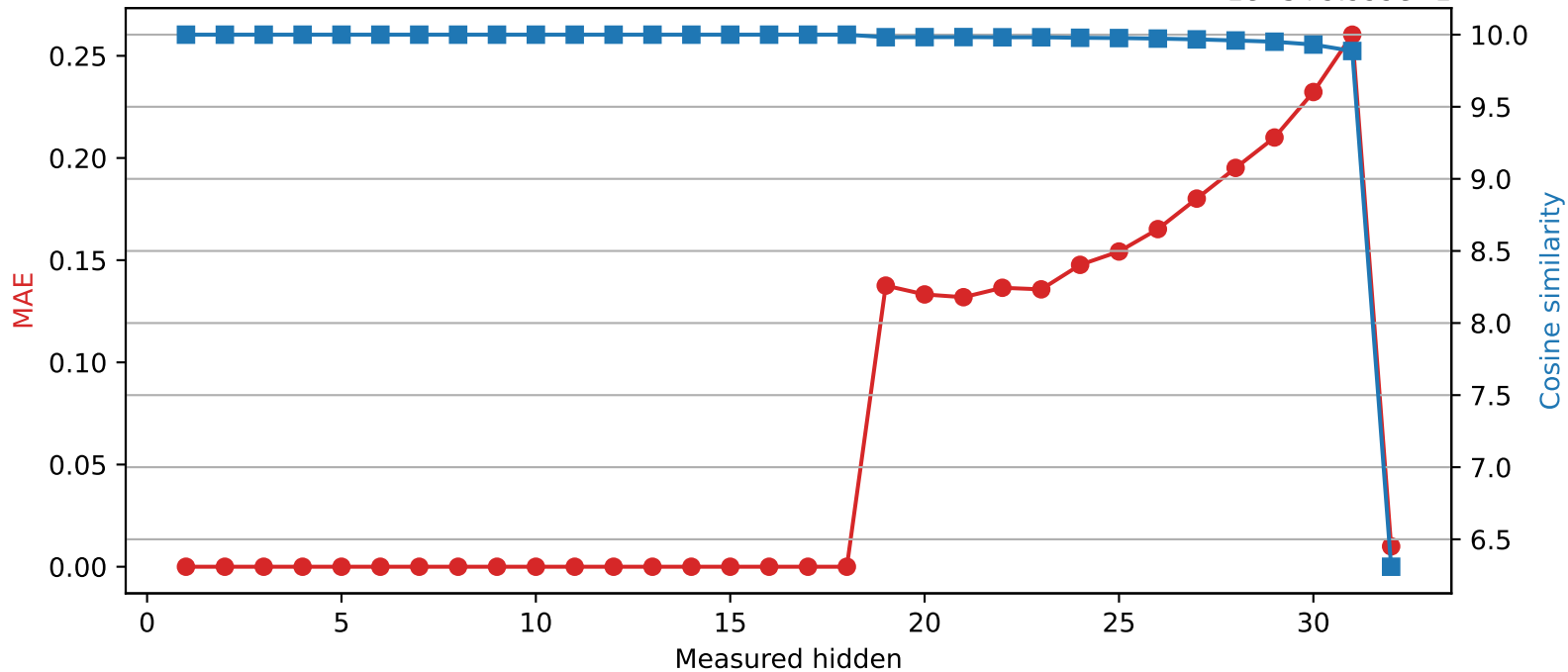
SmolLM2-360M | Quantized layer 18 | float32 → int8 1e-5 + 9.999e-1
