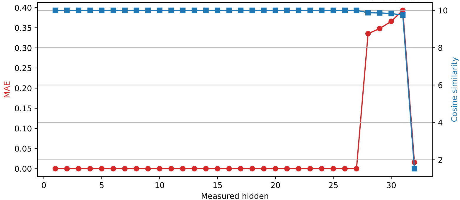
SmolLM2-360M | Quantized layer 27 | float32 → int8
