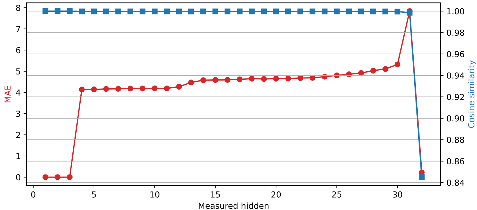
SmolLM2-360M | Quantized layer 3 | float64 → int8
