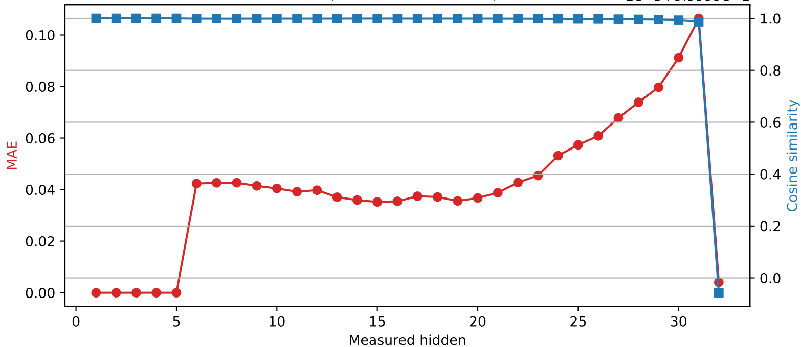
SmolLM2-360M | Quantized layer 5 | float64 → int8 1e-5 + 9.9999e-1
