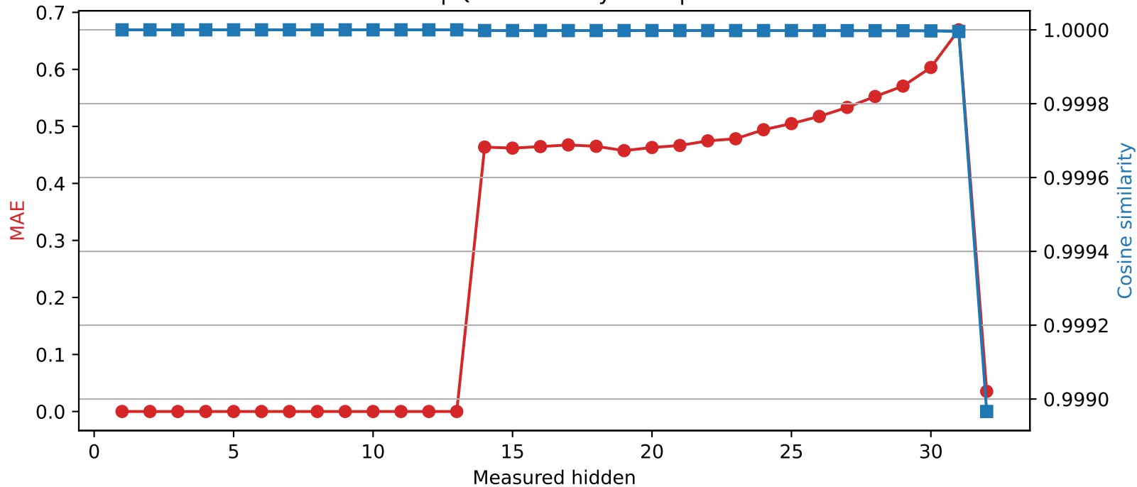
SmolLM2-360M | Quantized layer 13 | float64 → int8
