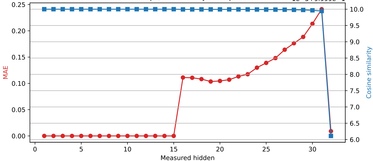
SmolLM2-360M | Quantized layer 15 | float64 → int8 1e-5+9.999e-1
