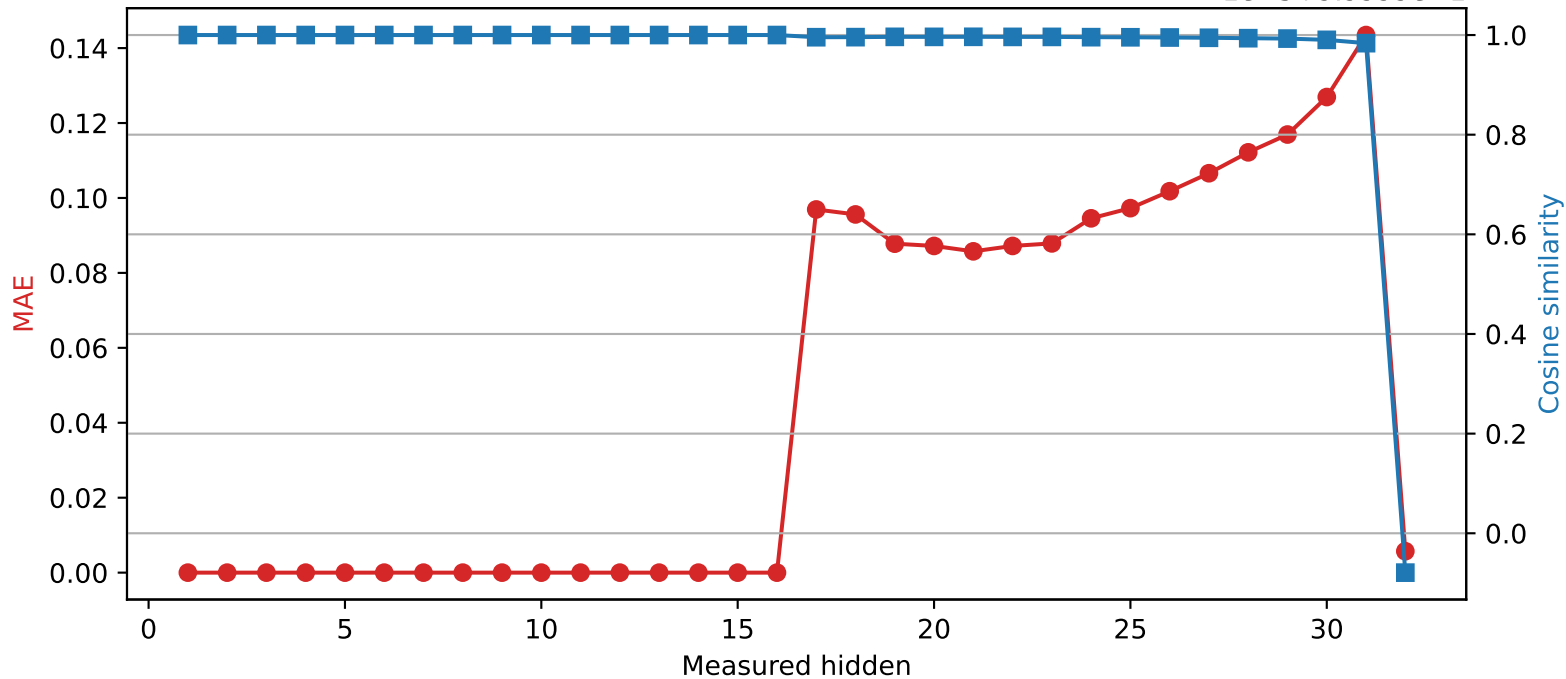
SmolLM2-360M | Quantized layer 16 | float64 \rightarrow int8 1e-5+9.9999e-1
