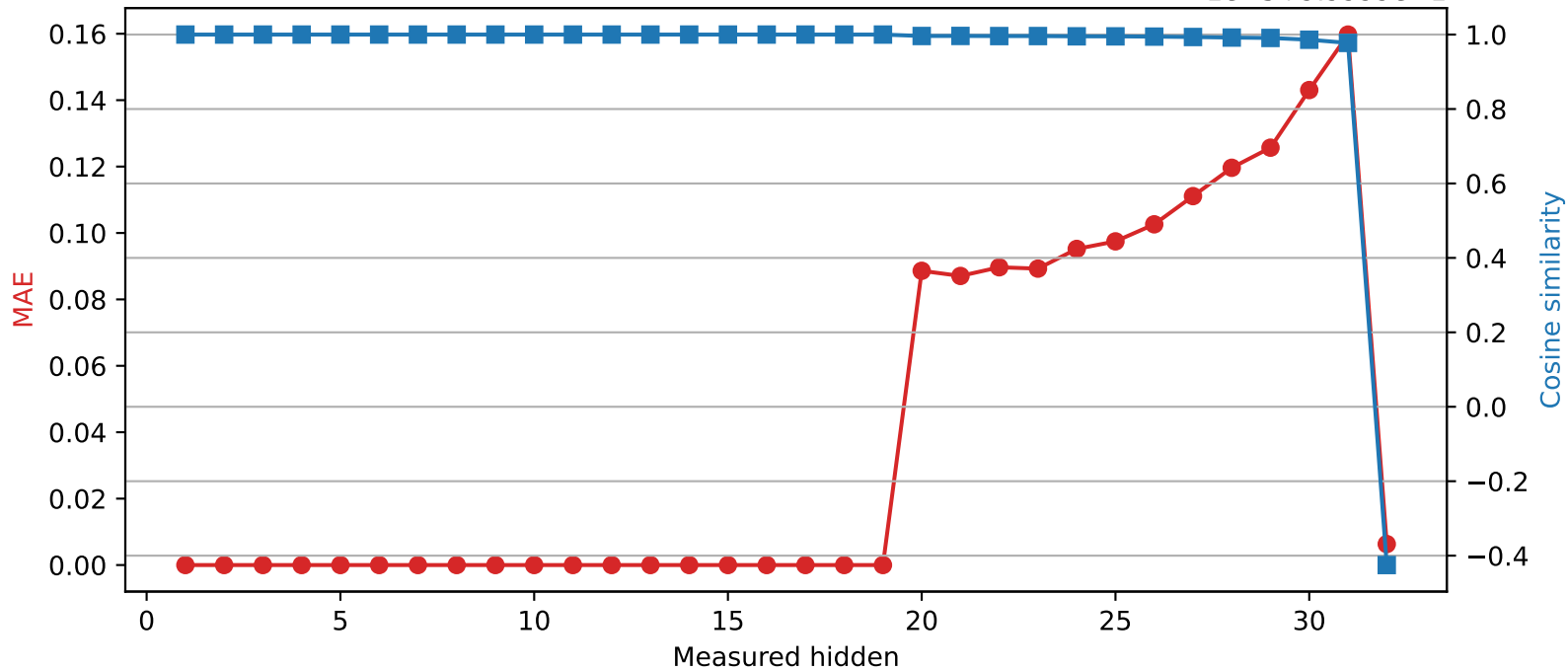
SmolLM2-360M | Quantized layer 19 | float64 \rightarrow int8 1e-5+9.9999e-1
