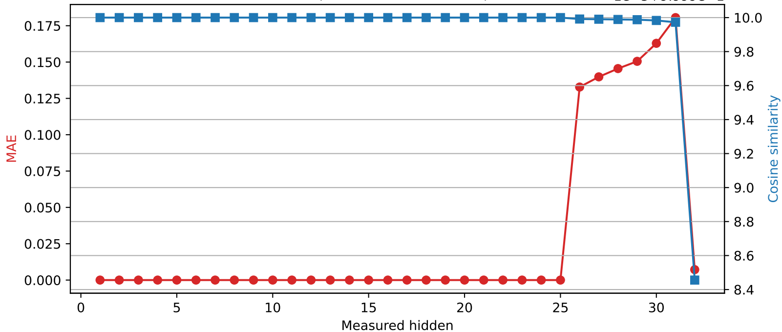
SmolLM2-360M | Quantized layer 25 | float64 → int8
