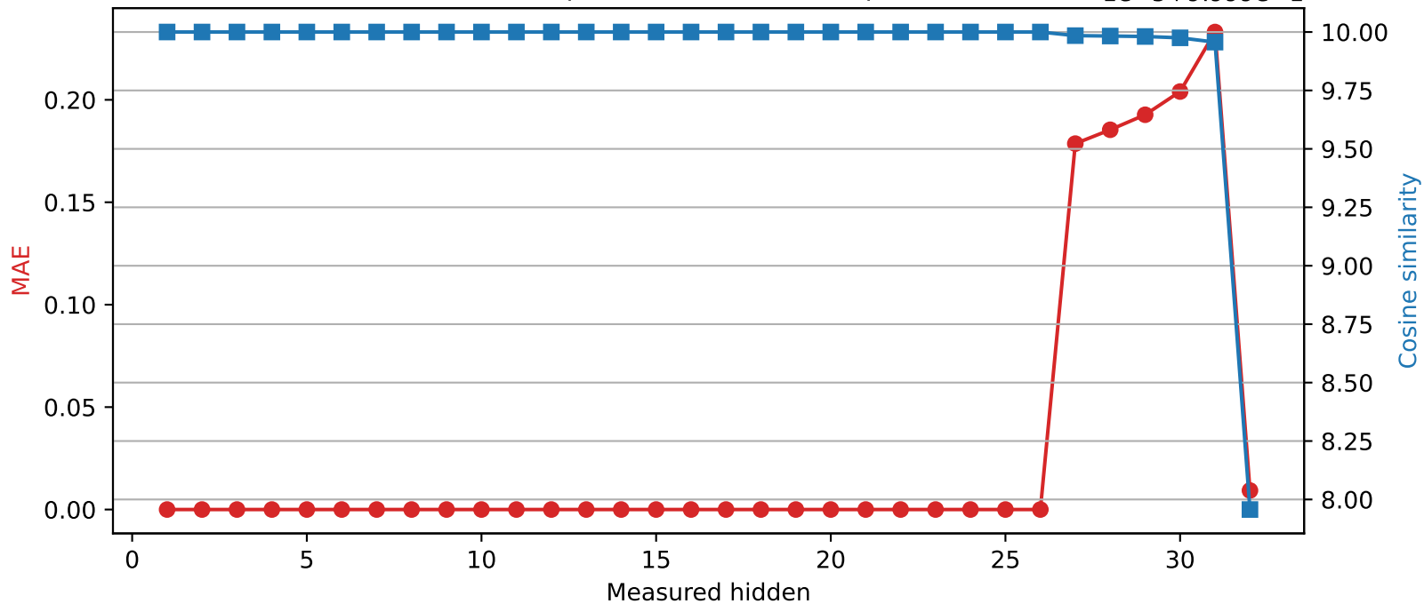
SmolLM2-360M | Quantized layer 26 | float64 → int8
