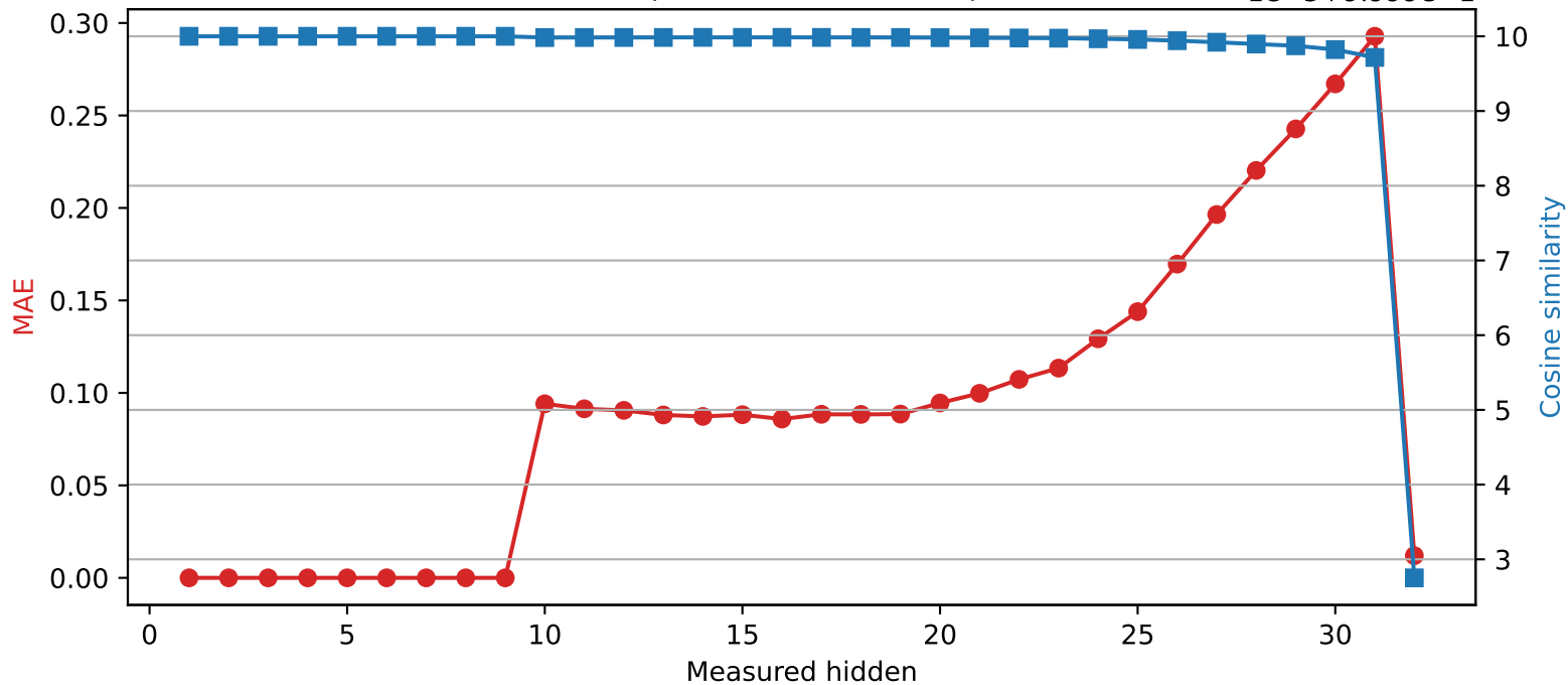
SmolLM2-360M | Quantized layer 9 | float64 → int8 1e-5+9.999e-1
