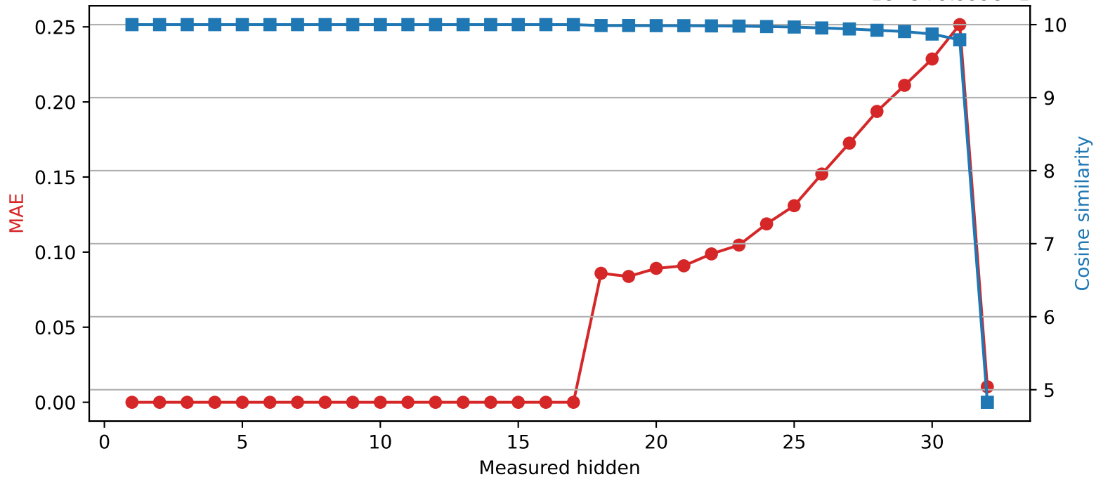
SmolLM2-360M | Quantized layer 17 | float64 → int8 1e-5+9.999e-1
