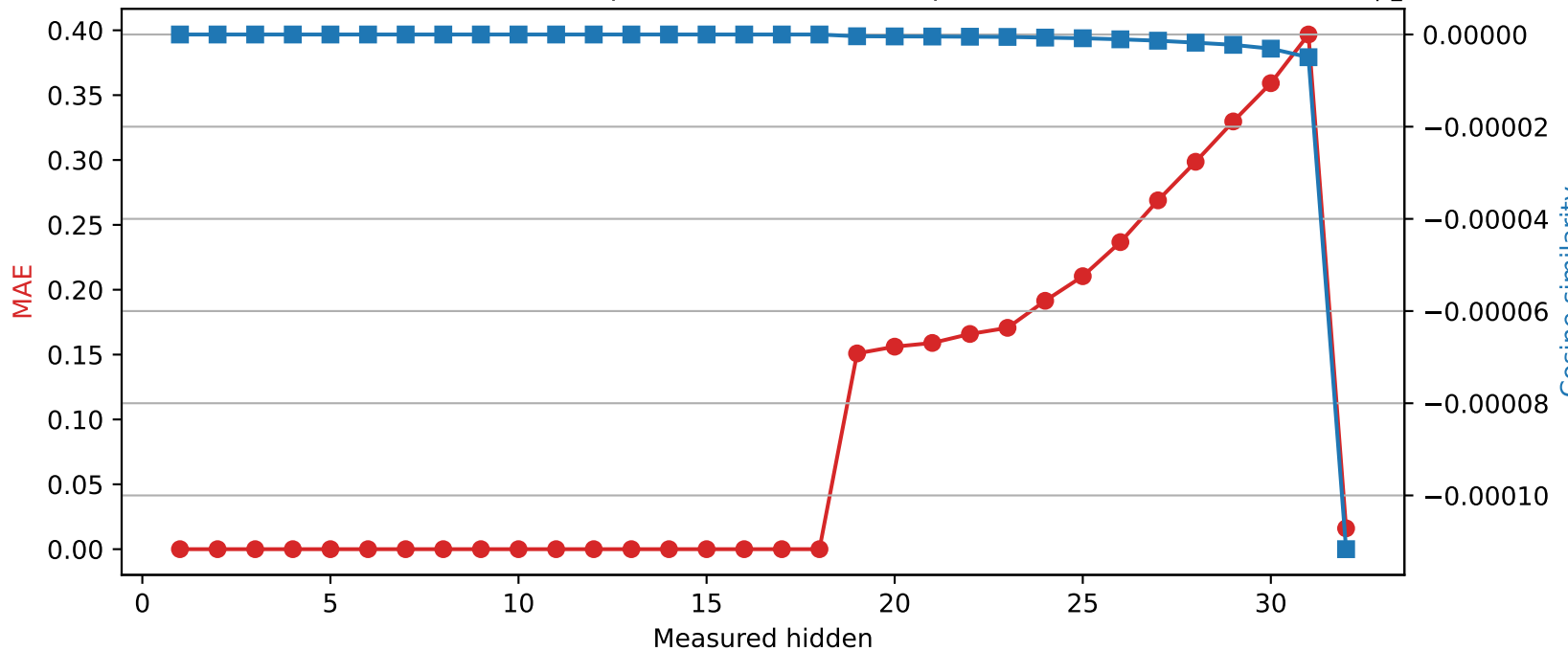
SmolLM2-360M | Quantized layer 18 | float64 → int8
