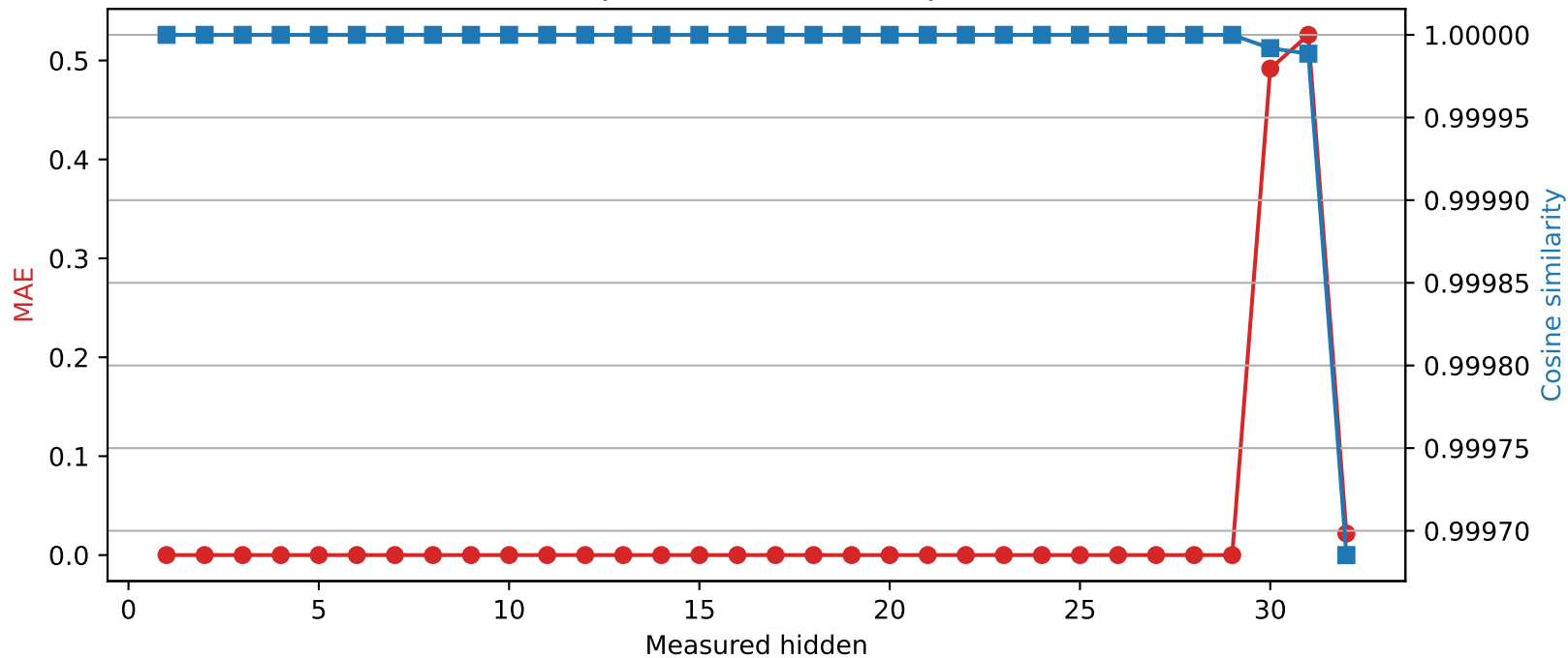
SmolLM2-360M | Quantized layer 29 | float64 → int8
