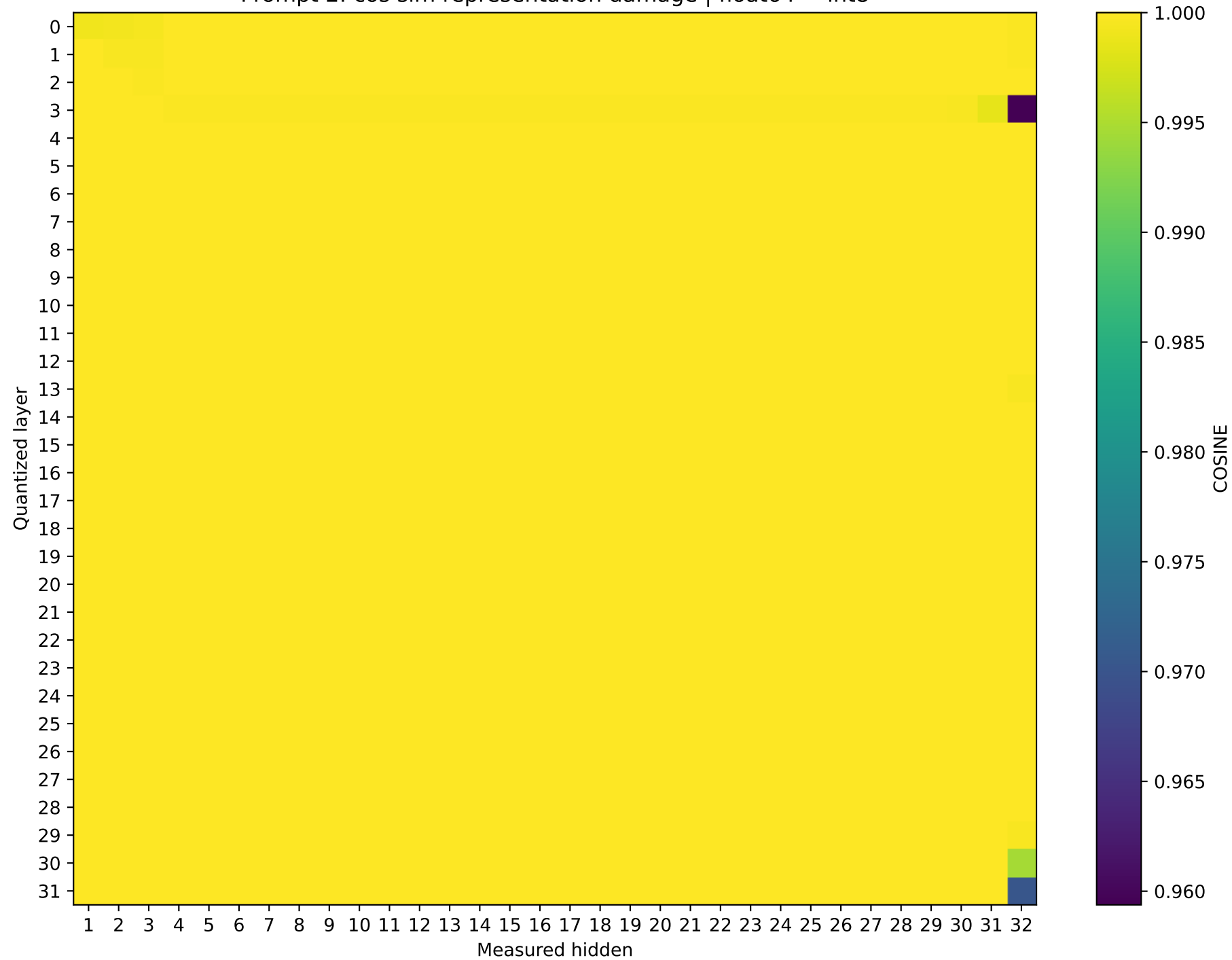
SmolLM2-360M Prompt 2: cos sim representation damage | float64 → int8
