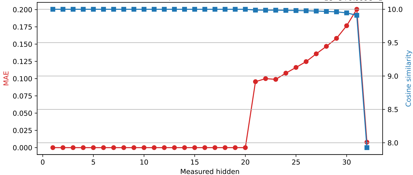
SmolLM2-360M | Quantized layer 20 | float64 → int8 1e-5+9.999e-1
