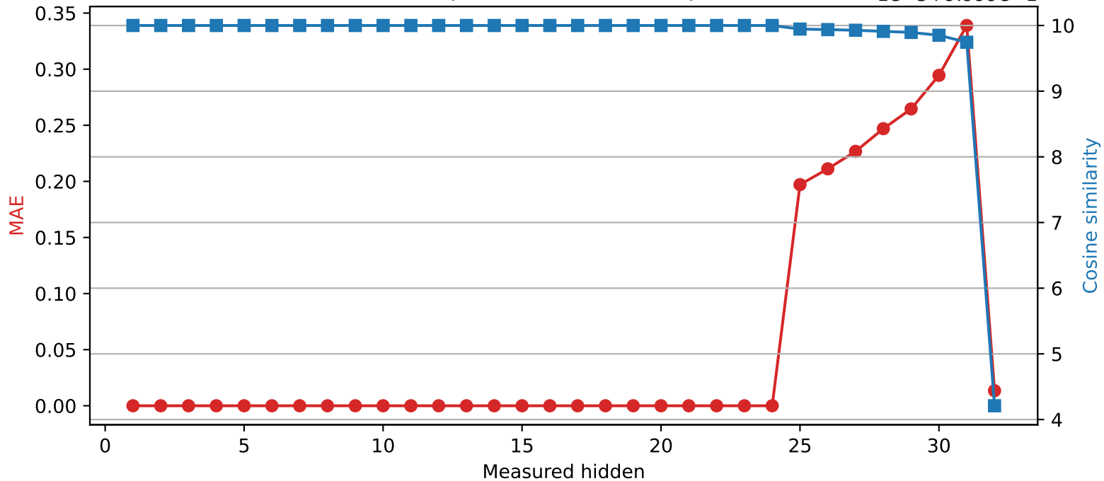
SmolLM2-360M | Quantized layer 24 | float64 → int8 1e-5 + 9.999e-1
