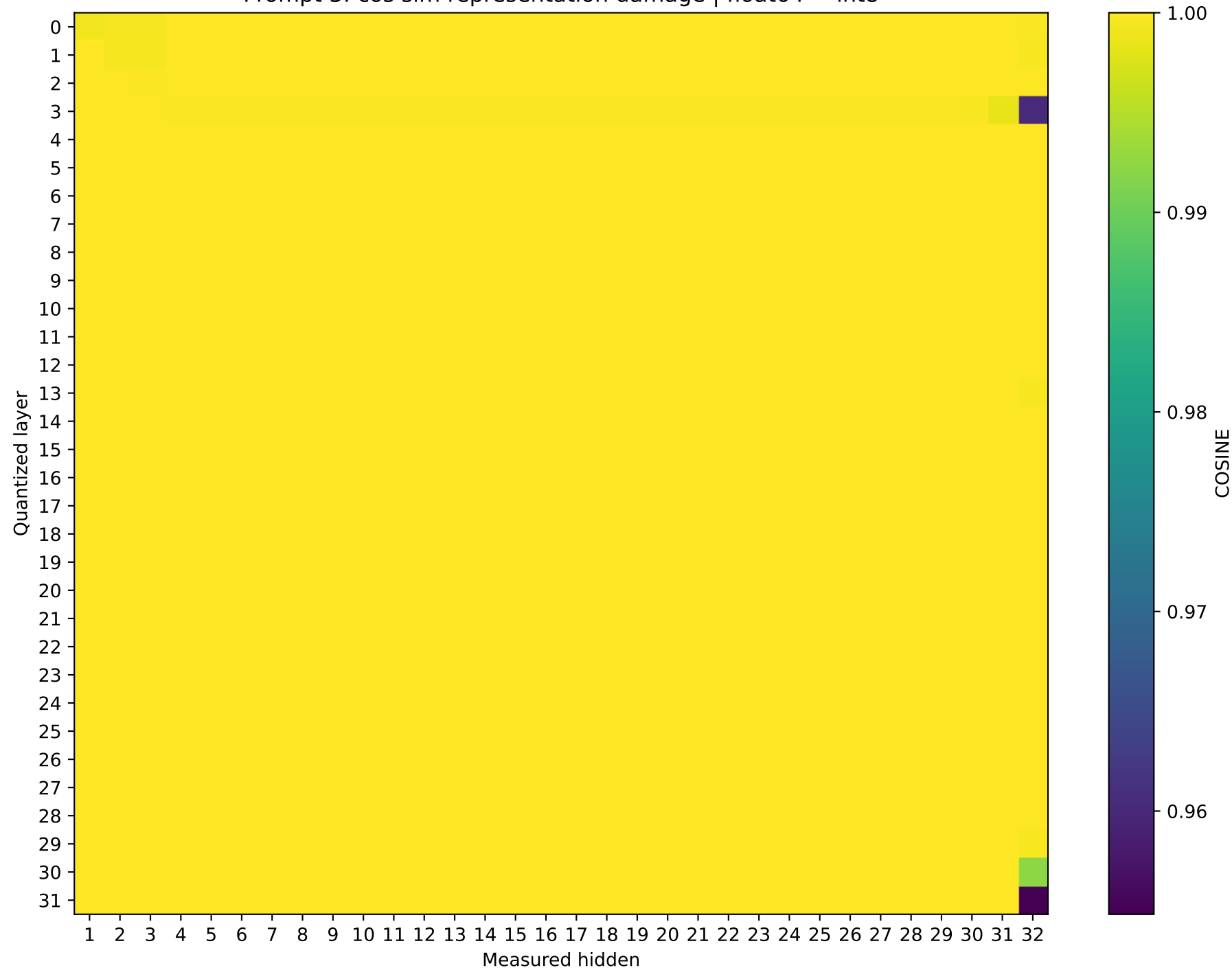
SmolLM2-360M Prompt 3: cos sim representation damage | float64 → int8
