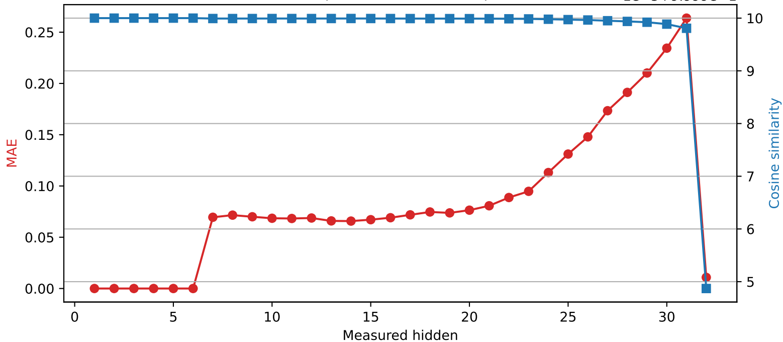
SmolLM2-360M | Quantized layer 6 | float64 → int8
