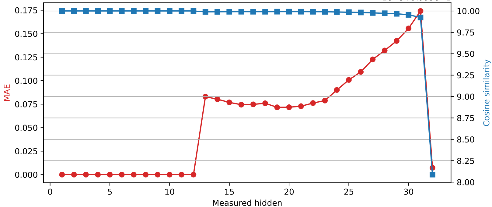
SmolLM2-360M | Quantized layer 12 | float64 → int8 1e-5+9.999e-1
