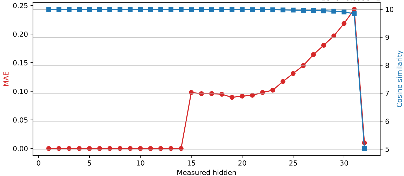
SmolLM2-360M | Quantized layer 14 | float64 → int8 1e-5+9.999e-1
