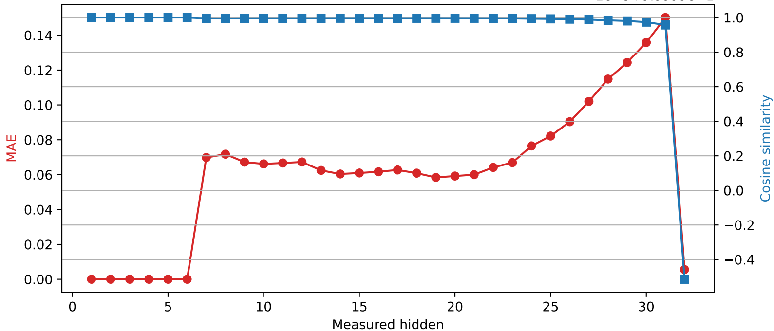
SmolLM2-360M | Quantized layer 6 | float64 → int8 1e-5 + 9.9999e-1
