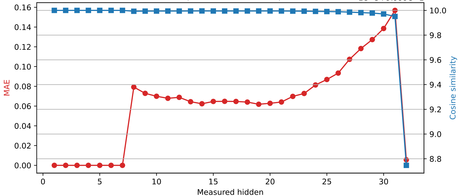
SmolLM2-360M | Quantized layer 7 | float64 → int8
