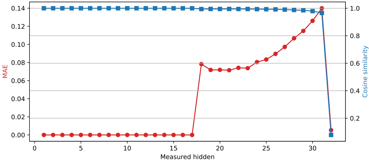
SmolLM2-360M | Quantized layer 17 | float64 → int8 1e-5 + 9.9999e-1
