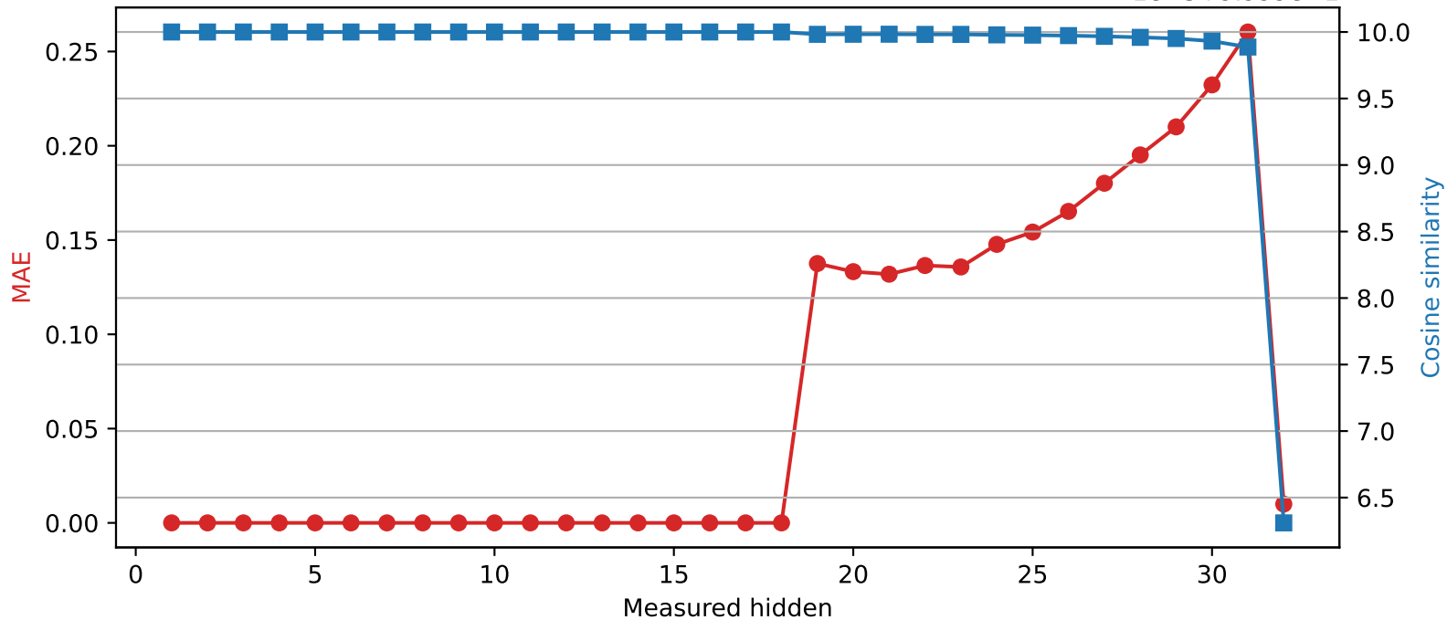
SmolLM2-360M | Quantized layer 18 | float64 → int8 1e-5+9.999e-1
