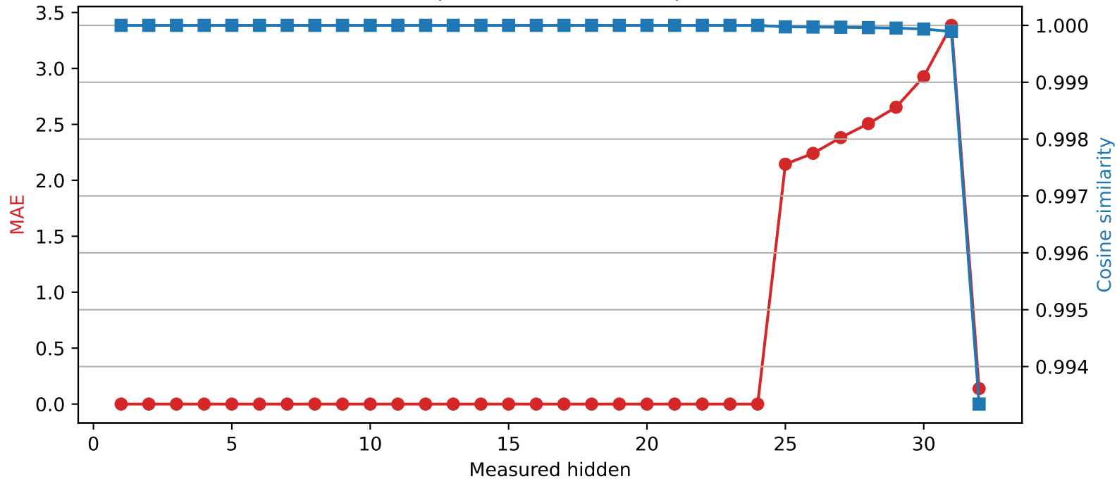
SmolLM2-360M | Quantized layer 24 | float16 \rightarrow int4
