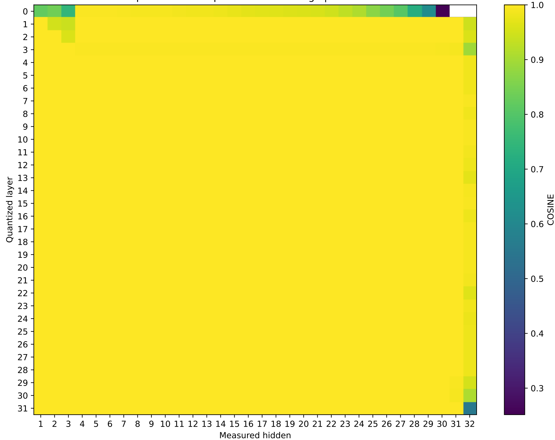
SmolLM2-360M Prompt 1: cos sim representation damage | float16 \rightarrow int4
