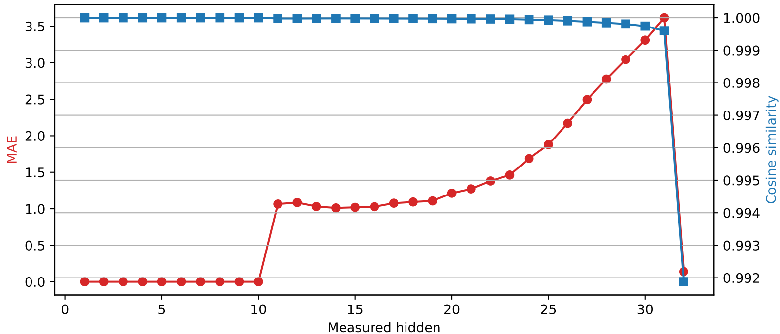
SmolLM2-360M | Quantized layer 10 | float16 → int4
